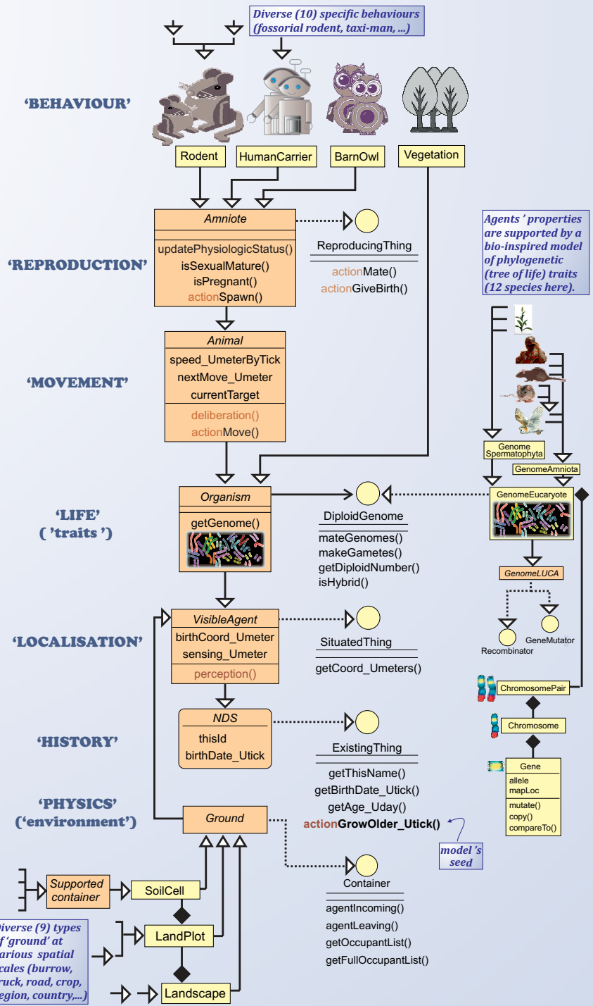
Figure 2: UML-based class diagram of the model's structure that emerged from the compilation of the eight case studies. Only the relevant methods, properties or relationships are presented
